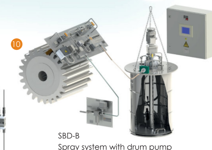
SBD-B Spray unit
